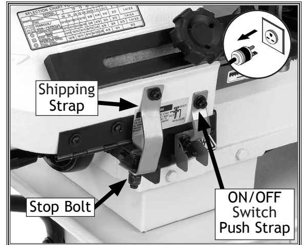
Figure 21. Shipping strap location.
